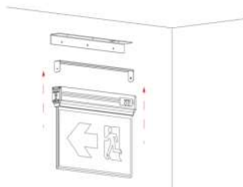
LX-S15N-1B / LX-S15R-1B
